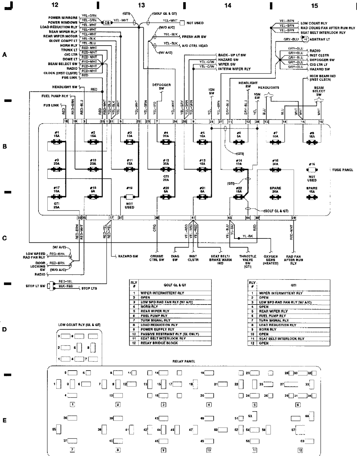
Fig. 4: Fuse Block
