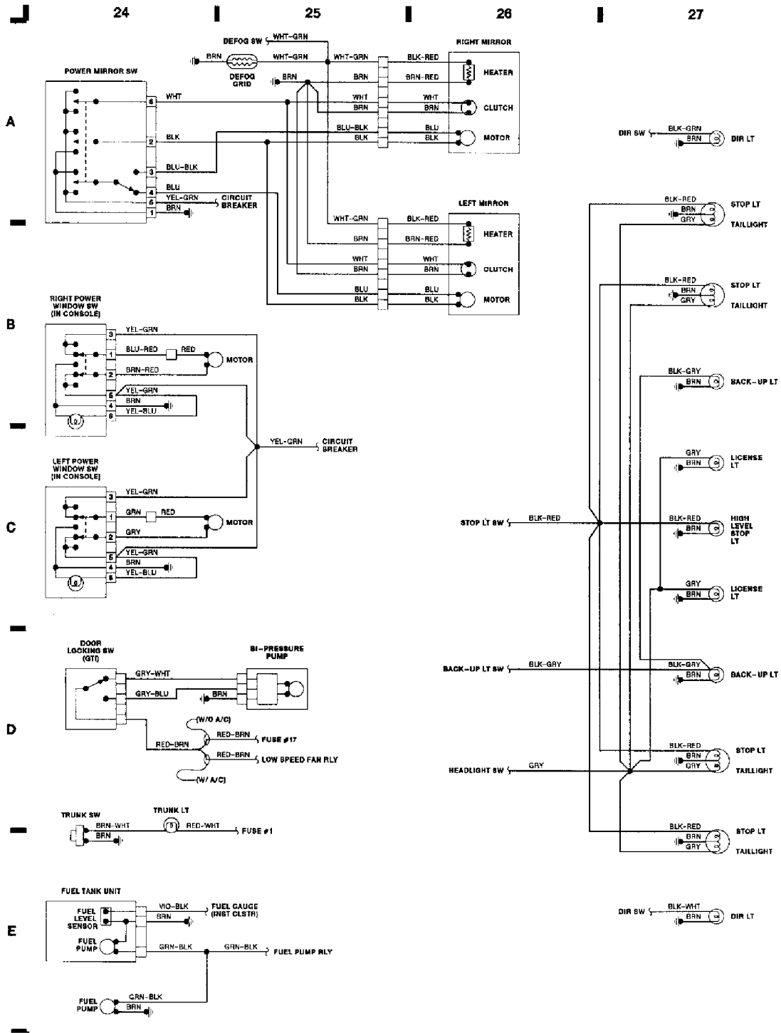
Fig. 7: Passenger Compartment & Taillights
