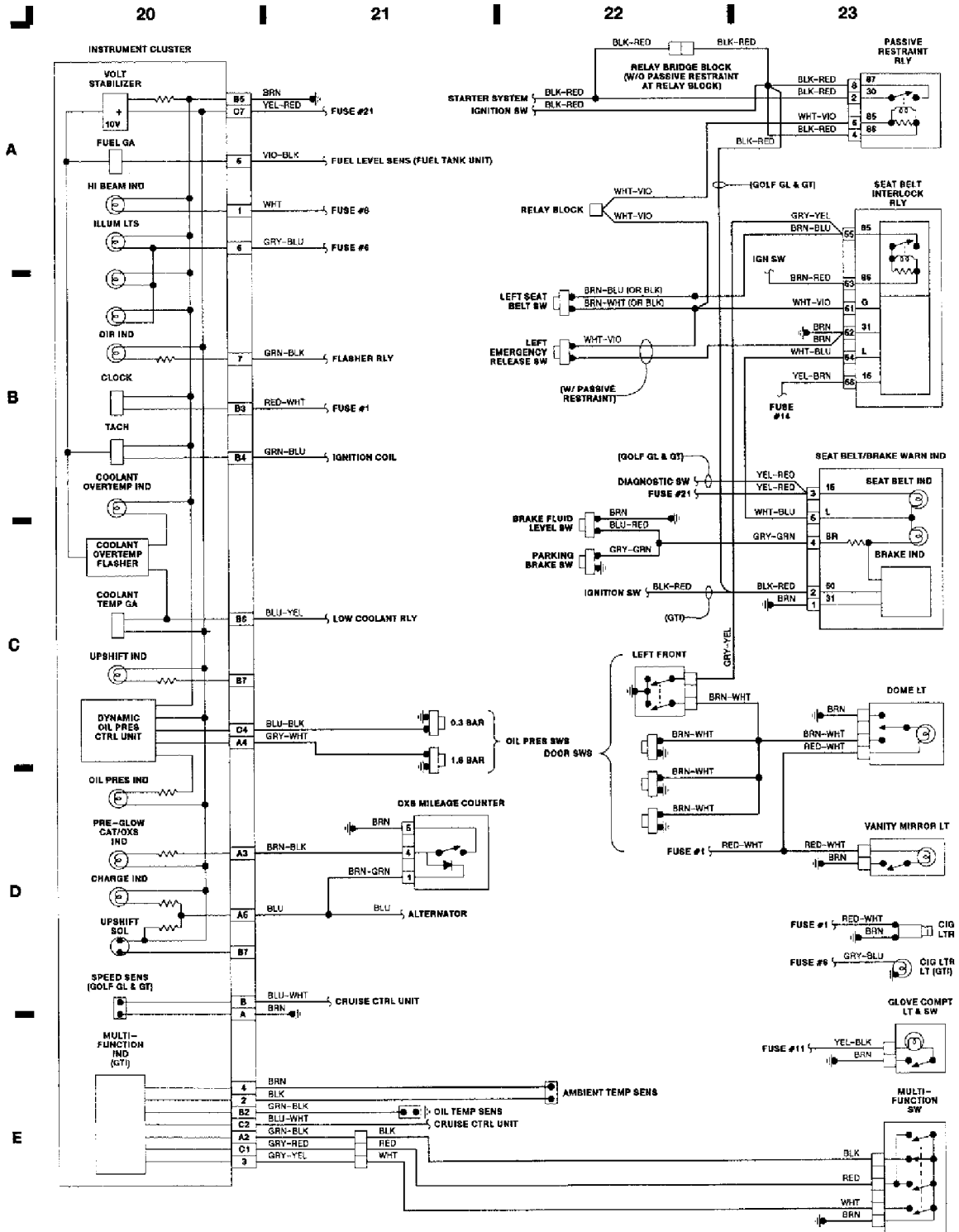
Fig. 6: Instrument Panel
