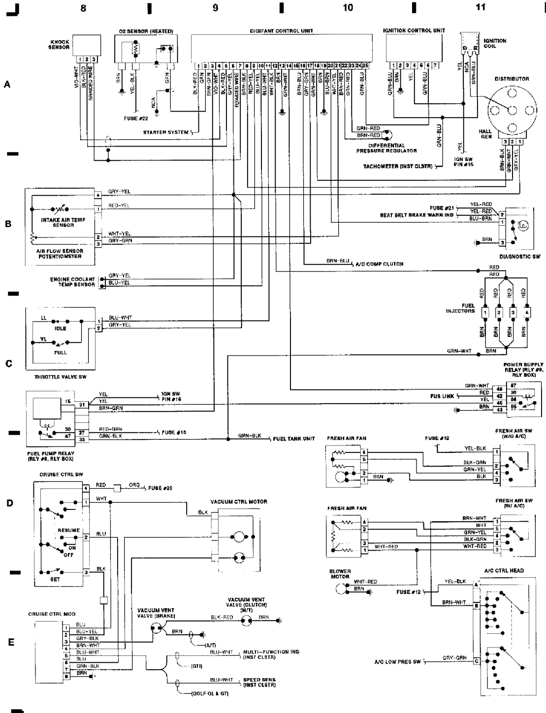
Fig. 3: Computer Engine Control (Golf)
