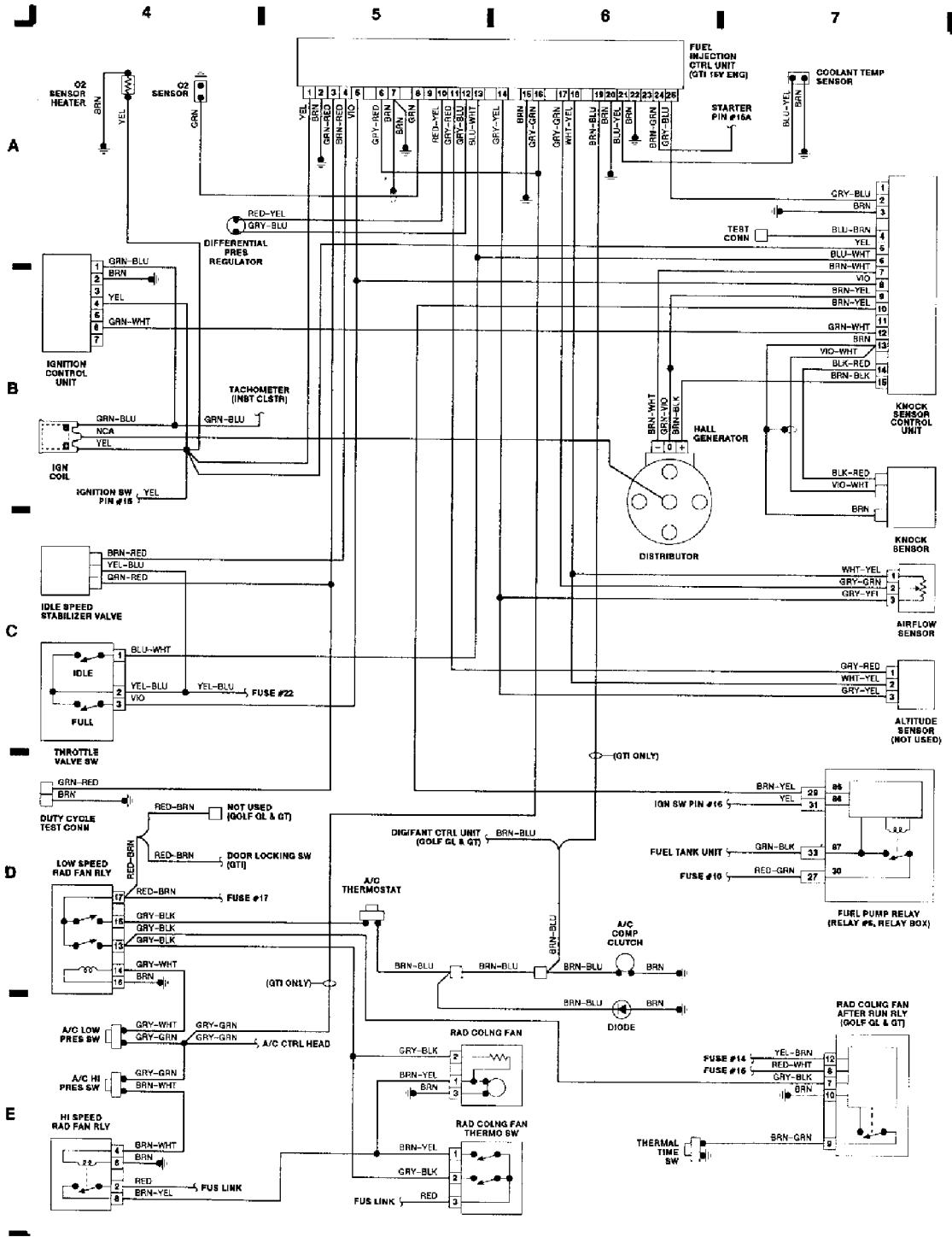
Fig. 2: Computer Engine Control (GTI 16-Valve Engine)
