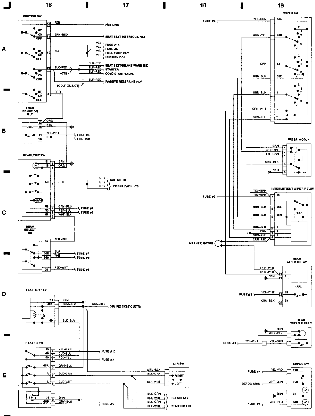
Fig. 5: Steering Column & Instrument Panel Switches
